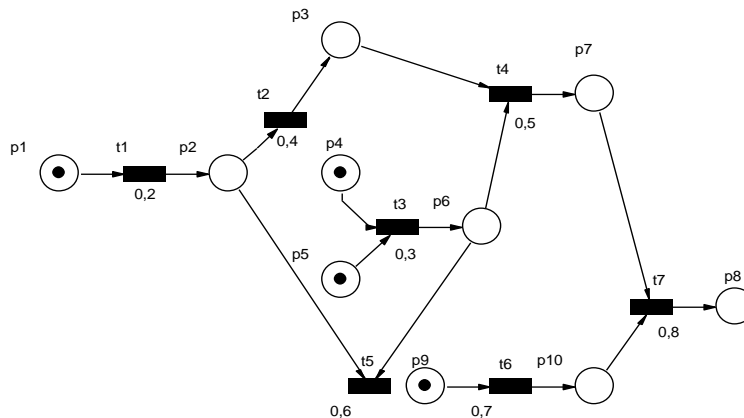
Figure 2: Fuzzy Petri net system of bank facilities
