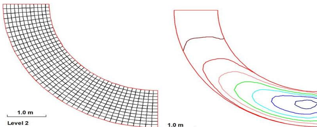
Fig 1: Plan view of the grid (left) for the bend. The water is flowing in from above and out to the right. The right figure shows a contour map of the secondary current angle. The dark blue value is -14 degrees. The dark red value is -2 degrees.
