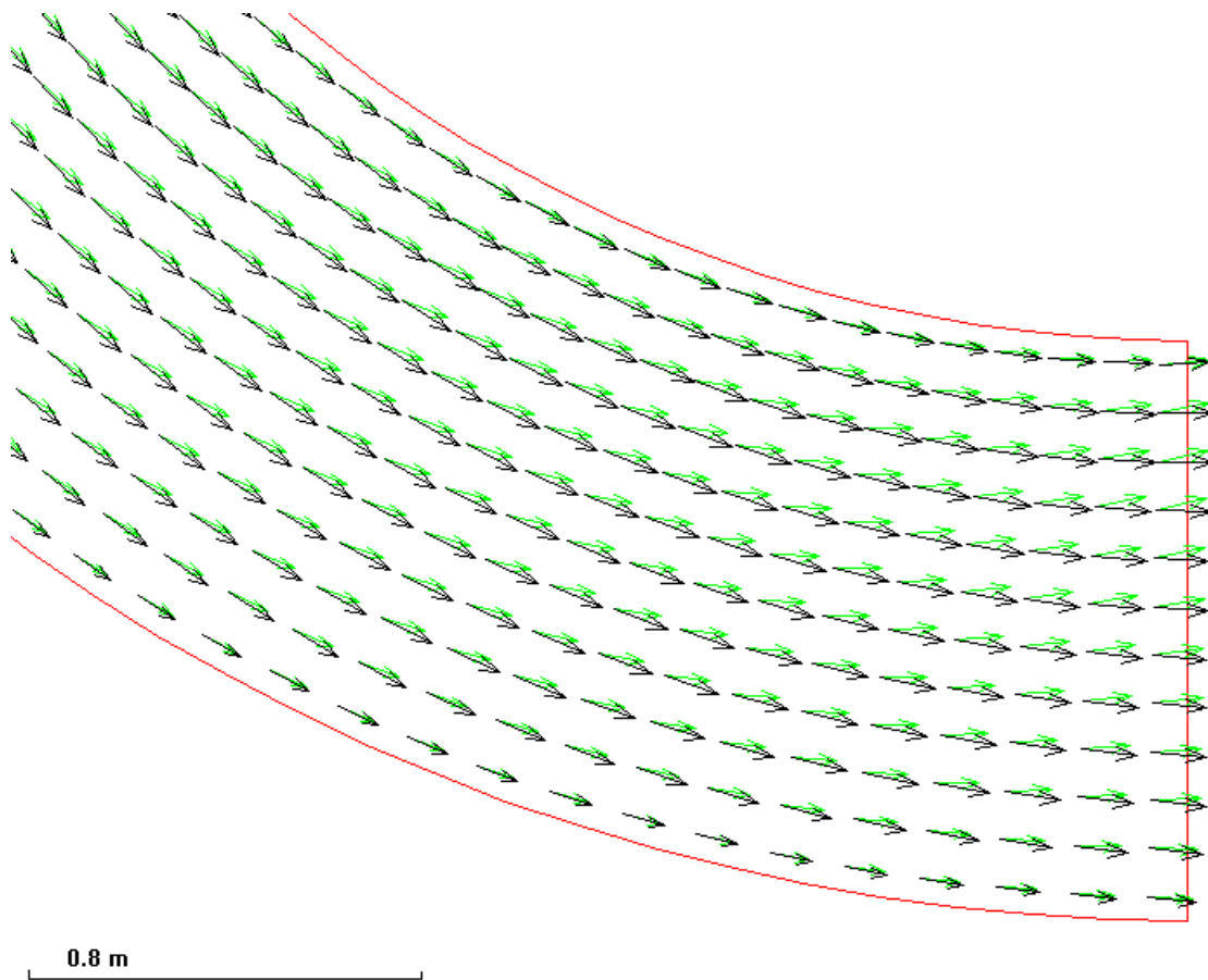
Fig 2: Velocity vectors at the surface and the bed for flow in a bend, showing the secondary current
